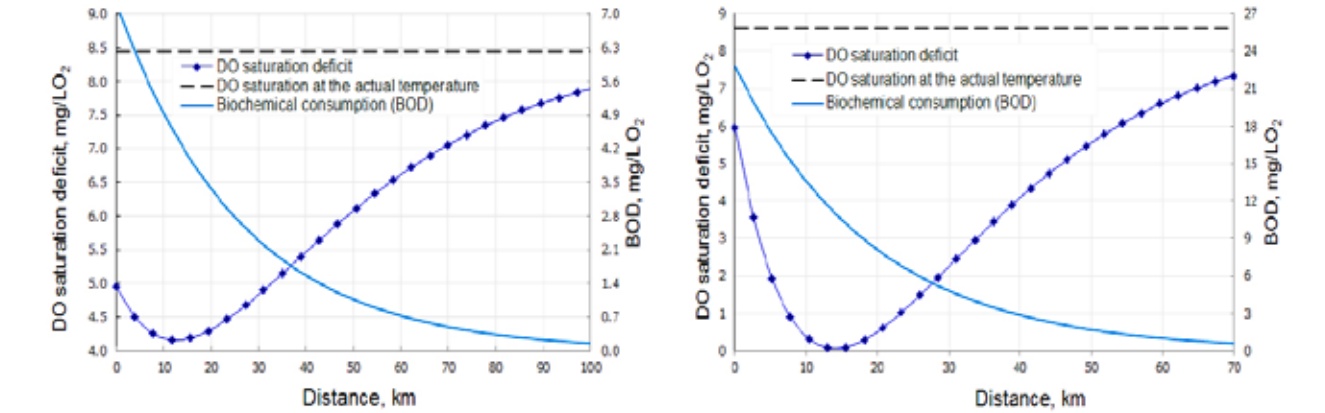
Fig. 4. The DO – BOD interaction in the Dniester River (left) and in the Reut River (right) The calculated model of DO – BOD interaction for the Soroca sampling station shows a considerable recovery potential of the Dniester River even when the initial BOD exceeds the 5th Water Quality Class. To pass the critical
